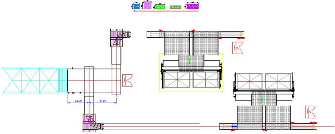
SIRLAMA BANDI SABİT ARABALI BUFFER / GLAZING LINE FIXED BOX BUFFER
