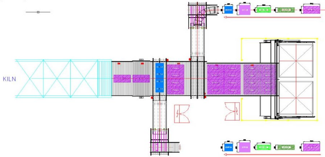
FIRIN GİRİŞİ SABİT ARABALI BUFFER / KILN ENTRANCE FIXED BOX BUFFER
