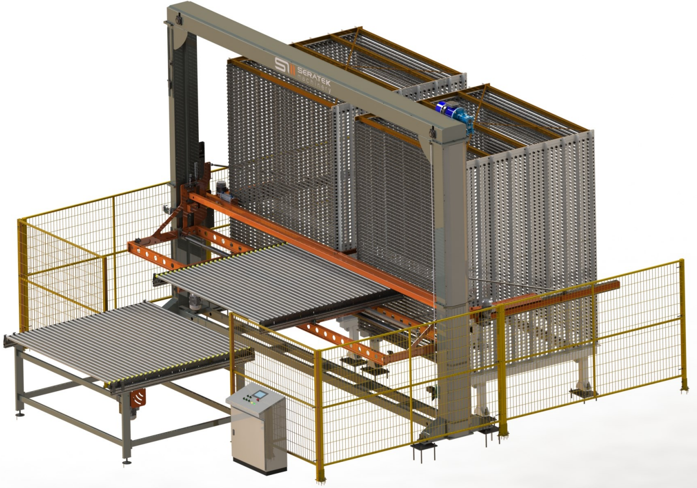
SABİT VEYA HAREKETLİ STOK ARABALI SİSTEM / FIXED OR MOVABLE STORAGE BOX SYSTEM
